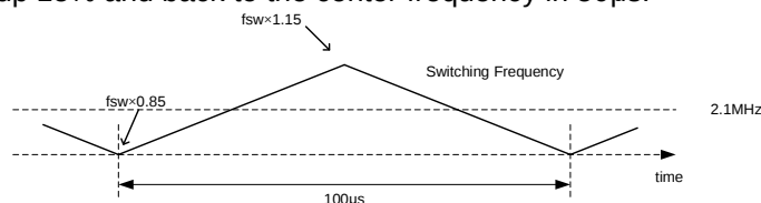
Figure5. Spread Spectrum
