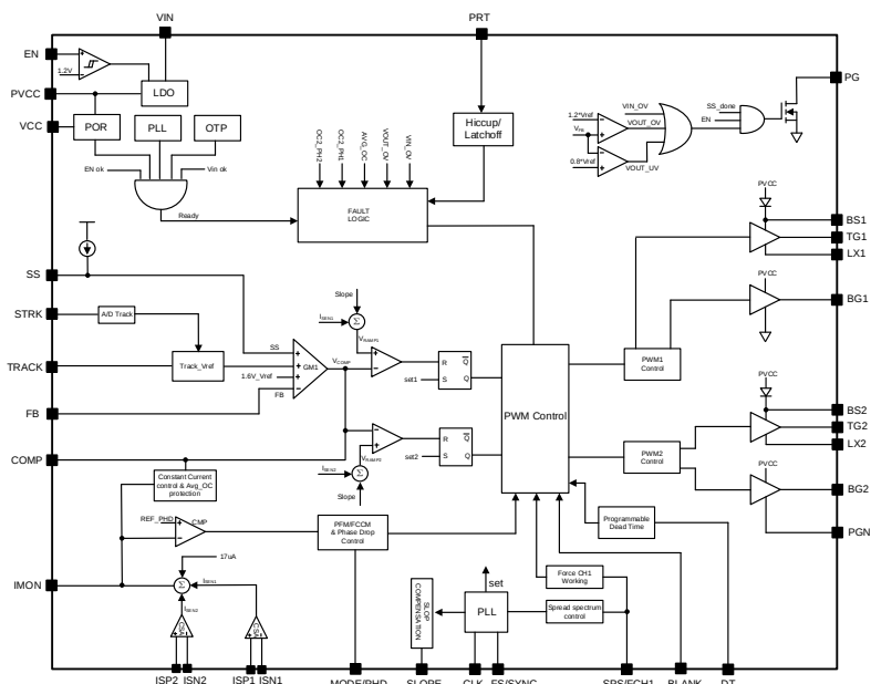
Figure 2. Block Diagram
