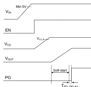
Figure3. Power On Sequence
