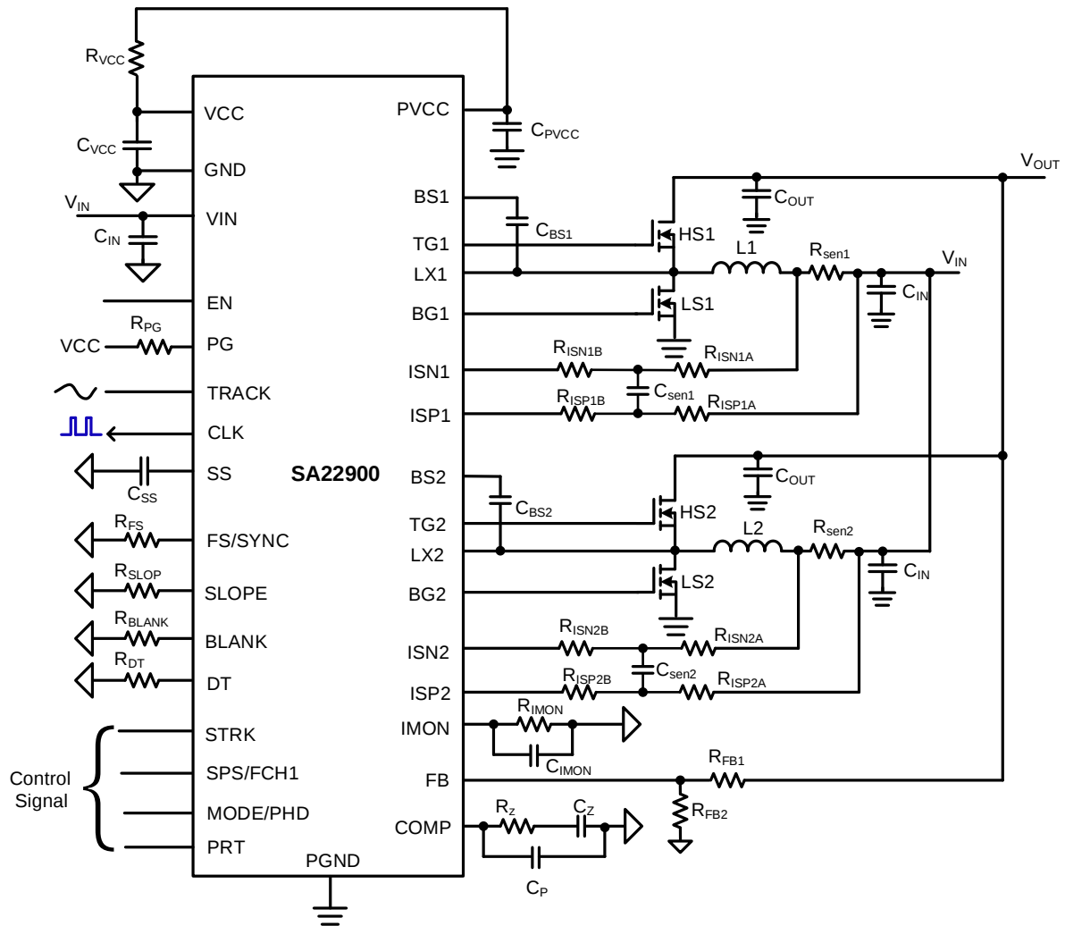
Figure 1a. Typical Application Circuit for Dual-phase Operation
