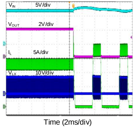
Pre-bias Function ( I_{OUT}=3A, FCCM )
