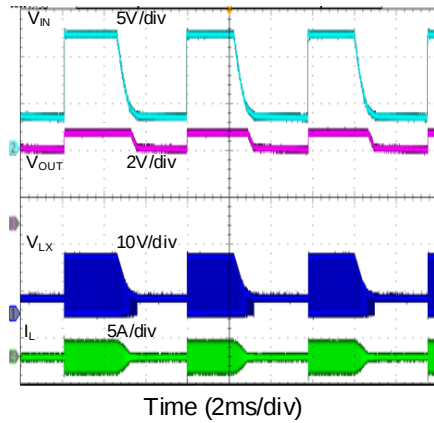
Pre-bias Function ( I_{OUT}=0A, FCCM )
