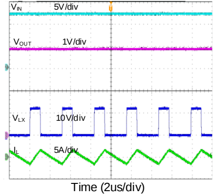
Steady States ( I_{OUT}=0A , PCCM)
