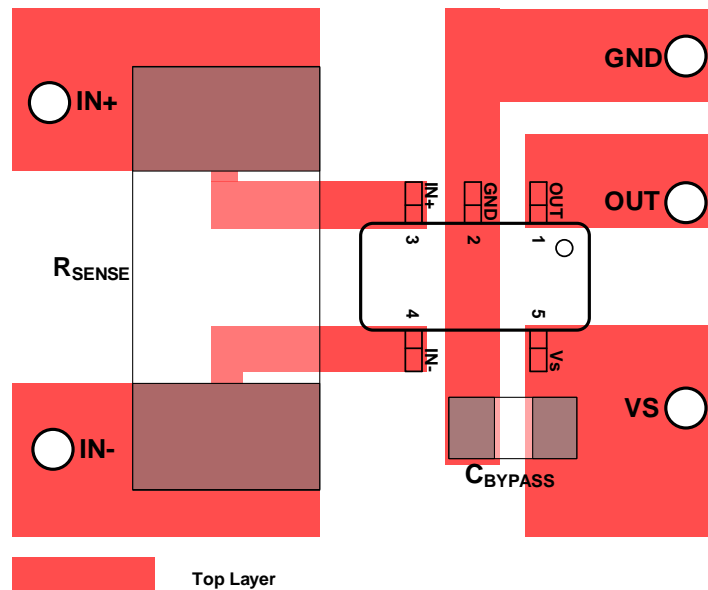
Figure 5. Recommended Layout
