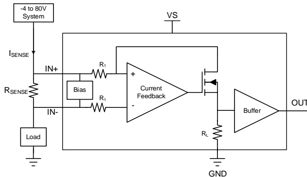
Figure 2. Unidirectional Application
