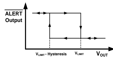
Figure 4. V_{LIMIT} Hysteresis
