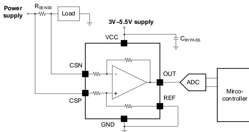
Figure 1. Typical Application
