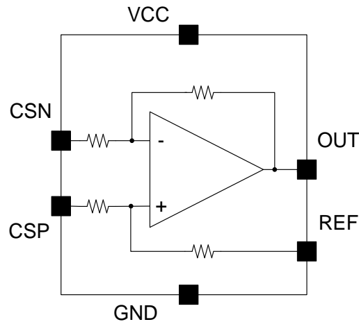
Figure 2. Block Diagram
