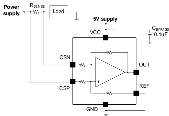
Figure 3. Unidirectional Current-sense Application
