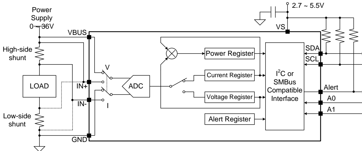
Figure 2. Block Diagram
