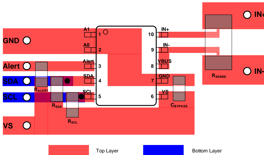
Figure 10. Recommended Layout
