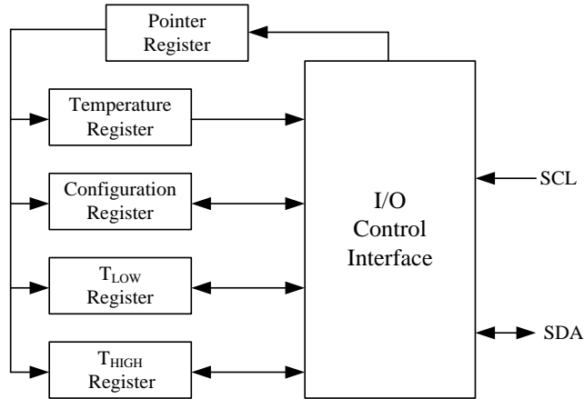
Figure 8. Internal Register Structure
