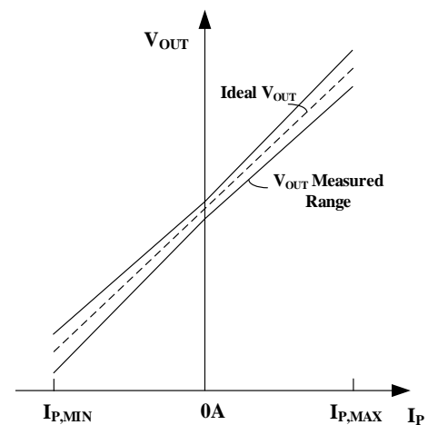
Figure 4. Linearity Error
