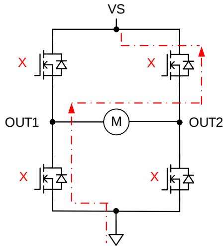
Figure 6. Coast-From Forward
