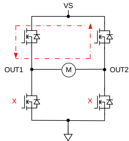
Figure 9. Brake-High-Side
