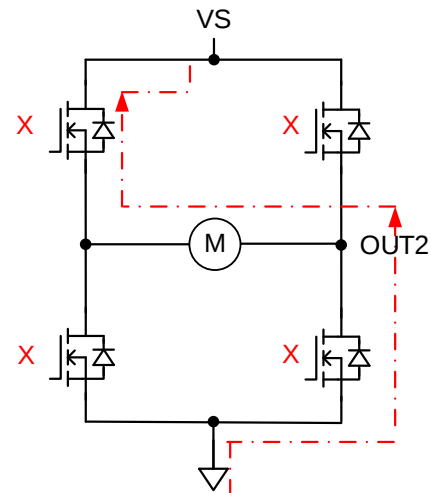
Figure 7. Coast-From Reverse
