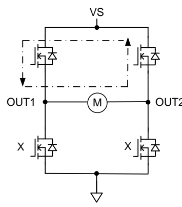
Figure 9. Brake-High-Side
