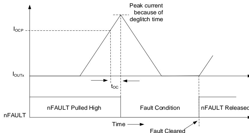
Figure 15. Over Current Protection
