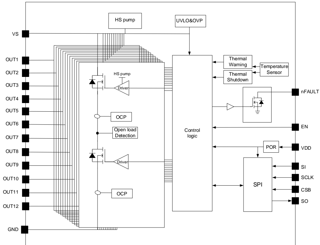
Figure 2. SA52122B Functional Block Diagram
