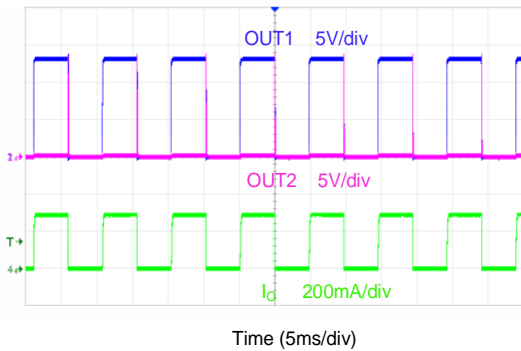
Passive Free-wheeling (VS=13.5V I o =300mA Duty=50% Frequency=100Hz)
