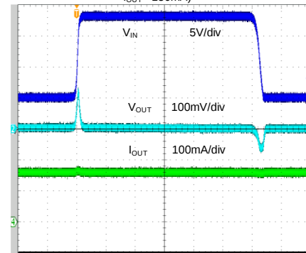
Line Transient ( V_{IN}=5V \sim 18V \sim 5V , V_{OUT}=3.3V , C_{IN}=10\mu F , C_{OUT}=4.7\mu F , I_{OUT}=150mA )
