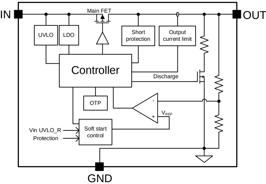
Figure2. Block Diagram
