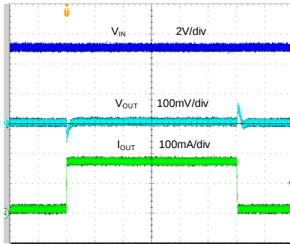
Load Transient ( V_{IN}=5V , V_{OUT}=3.3V , C_{IN}=10\mu F , C_{OUT}=4.7\mu F , I_{OUT}=10mA \sim 150mA \sim 10mA )
