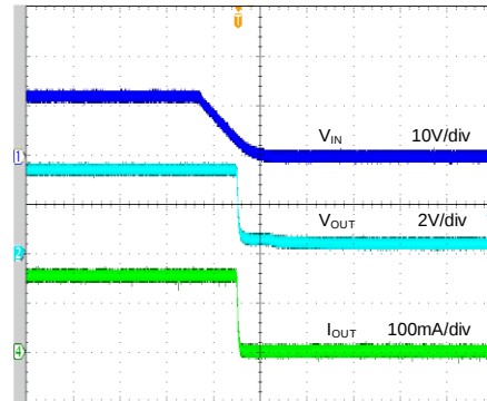
Shutdown from V_{IN} ( V_{IN}=12V , V_{OUT}=3.3V , I_{OUT}=150mA , C_{IN}=10\mu F , C_{OUT}=4.7\mu F )
