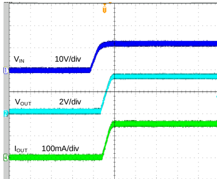
Startup from V_{IN} ( V_{IN}=12V , V_{OUT}=3.3V , I_{OUT}=150mA , C_{IN}=10\mu F , C_{OUT}=4.7\mu F )
