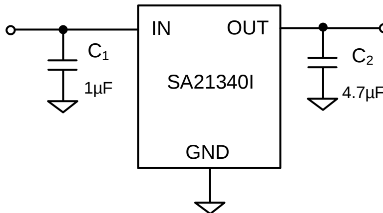
Figure1. Schematic Diagram
