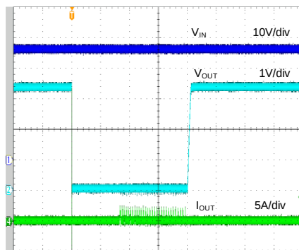
Short Protection ( V_{IN}=36V , V_{OUT}=3.3V , C_{IN}=10\mu F , C_{OUT}=4.7\mu F )
