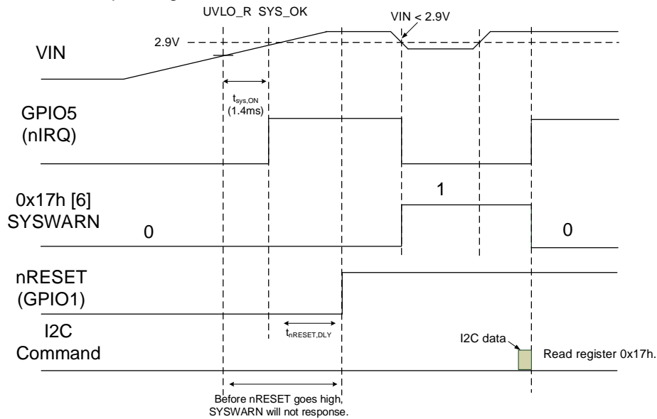
Figure 12. Timing Diagram of nIRQ (SYSWARN)
