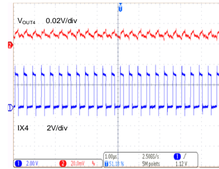
Buck4 Waveforms (FCCM Mode, V_{IN}=3.3V , V_{OUT4}=1.2V , L=0.47\mu H , C_{OUT}=22\mu F , I_{OUT}=2A )
