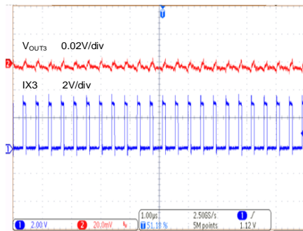
Buck3 Waveforms (FCCM Mode, V_{IN}=3.3V , V_{OUT3}=0.8V , L=0.47\mu H , C_{OUT}=22\mu F , I_{OUT}=4A )
