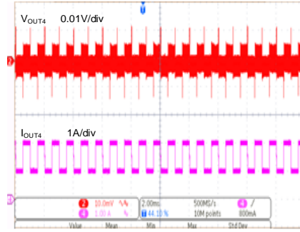
Buck4 Load Transient
