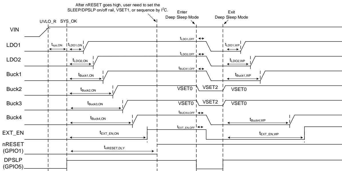
Figure 20. Conceptual of Sequence for Enter/Exit DPSLP Mode
