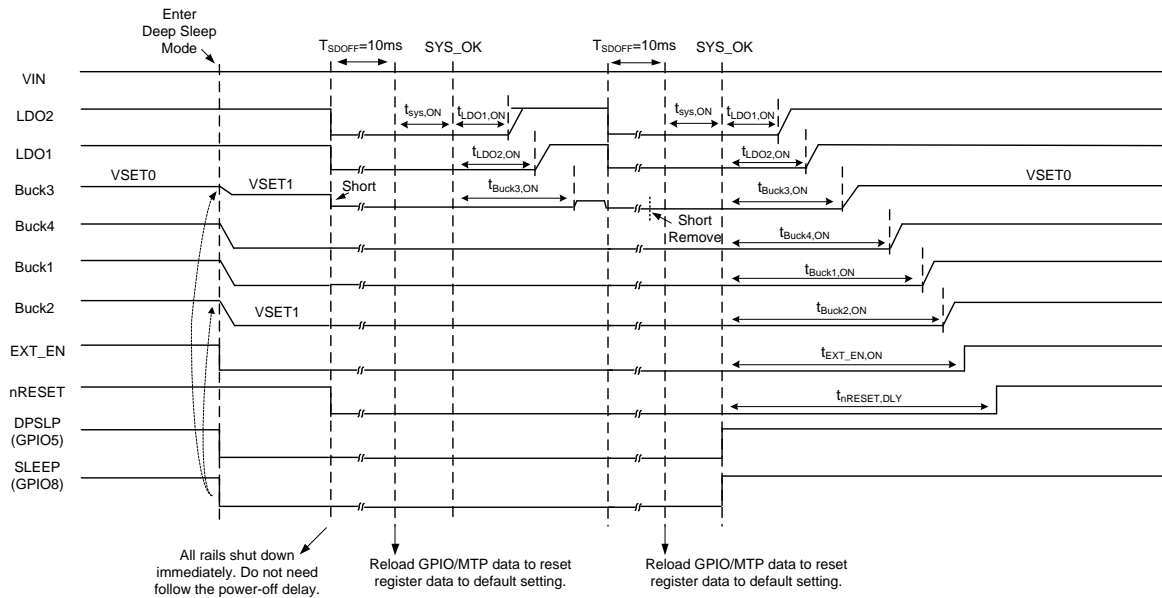
Figure 24. Conceptual of Buck3 Occurring Output Short Circuit Event in Deep Sleep Mode
