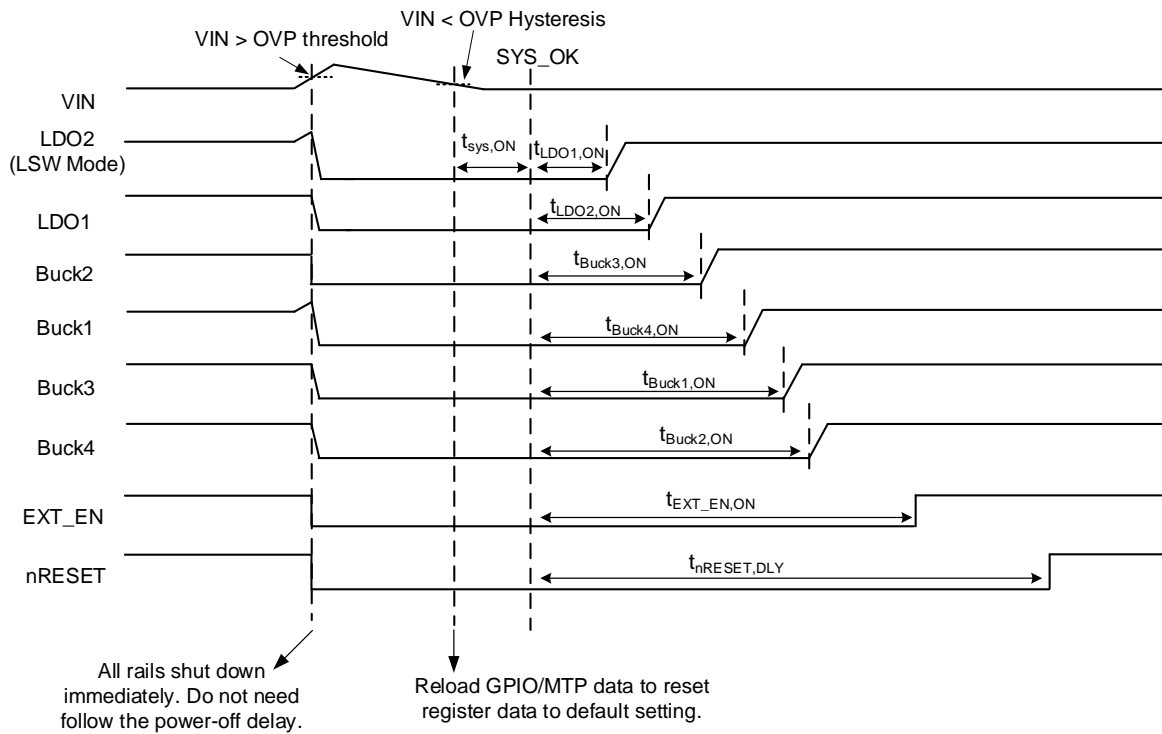
Figure 25. Conceptual of INPUT over Voltage Protection Mechanism
