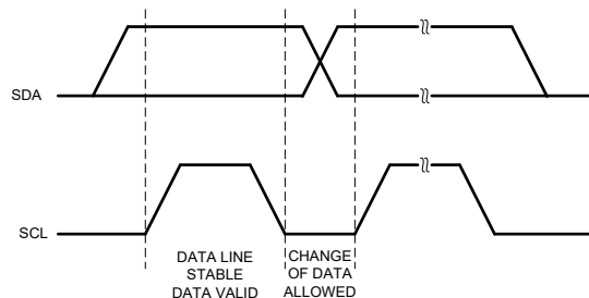
Figure 30. Data Validity
