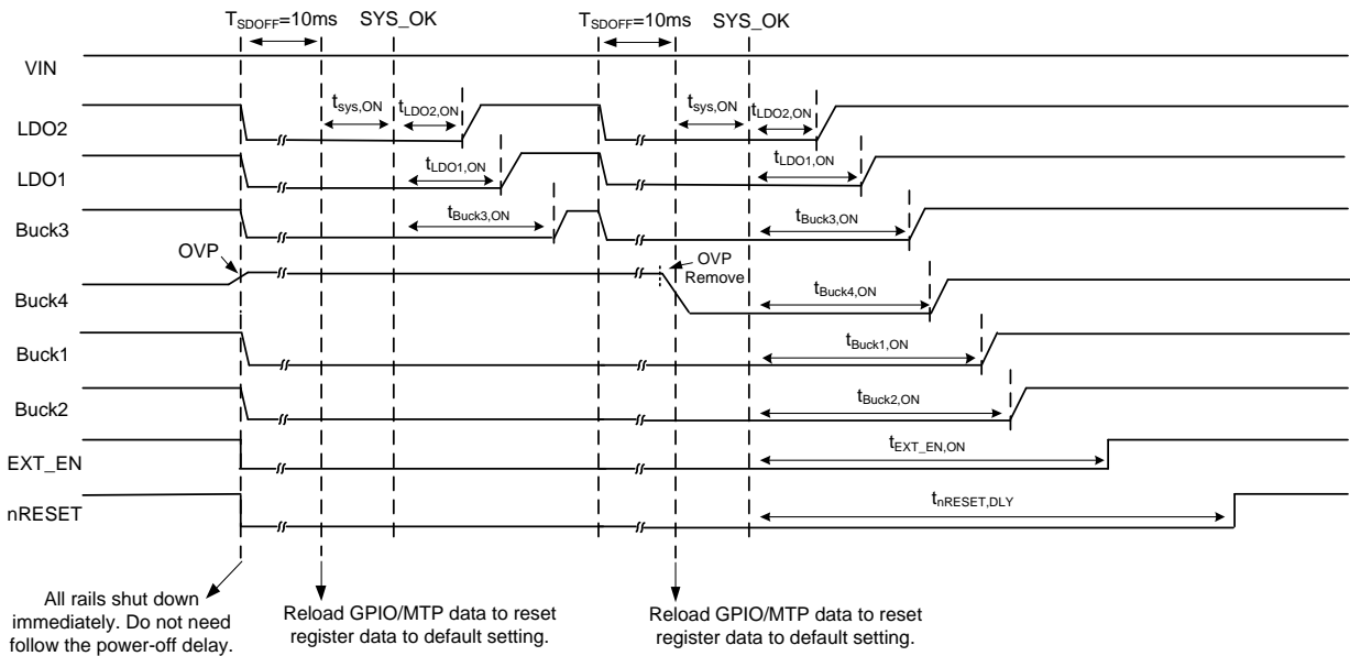
Figure 23. Conceptual of Buck4 Occurring Output over Voltage Event in Active Mode
