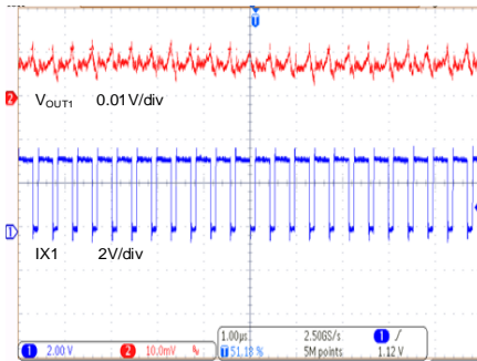
Buck1 Waveforms (FCCM Mode, V_{IN}=3.3V , V_{OUT1}=2.5V , L=0.47\mu H , C_{OUT}=22\mu F , I_{OUT}=4A )
