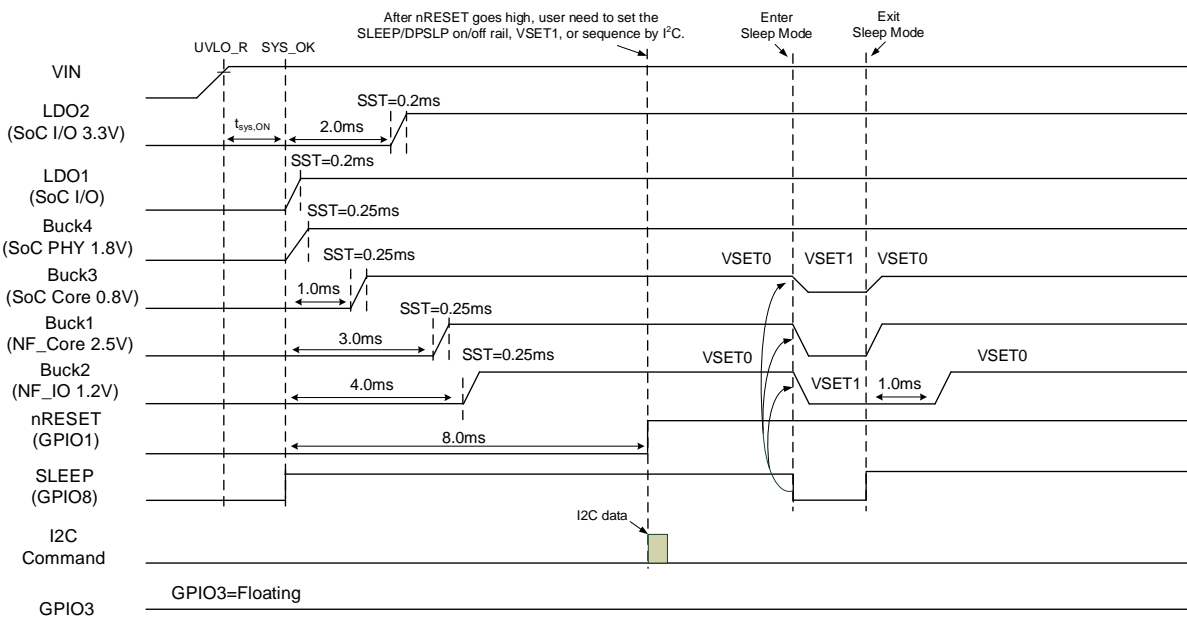
Figure 19. SLEEP Sequence for Application B
