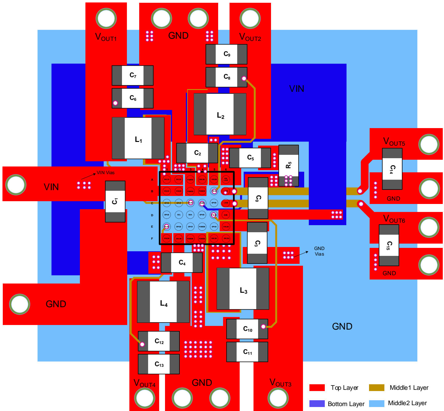
Figure 27. Suggested PCB Layout
