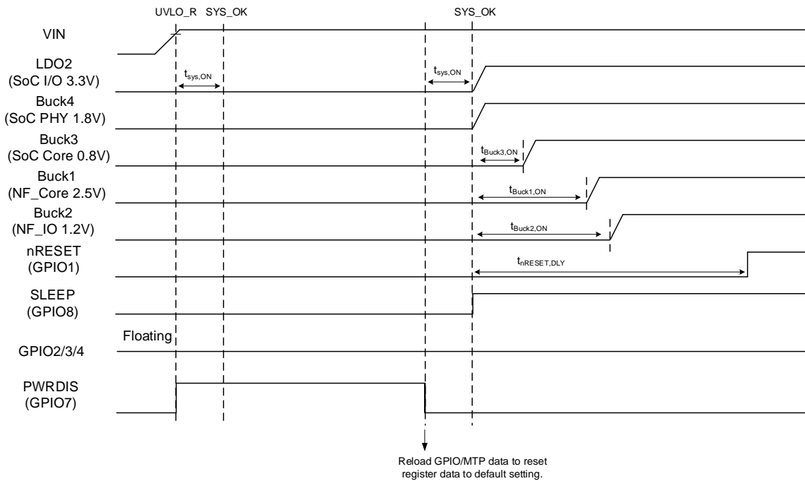
Figure 16. Conceptual of Timing Diagram for PWRDIS during V_{IN} Power-on
