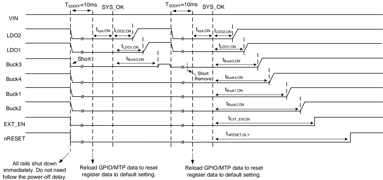
Figure 22. Conceptual of Buck3 Occurring Output Short Circuit Event in Active Mode
