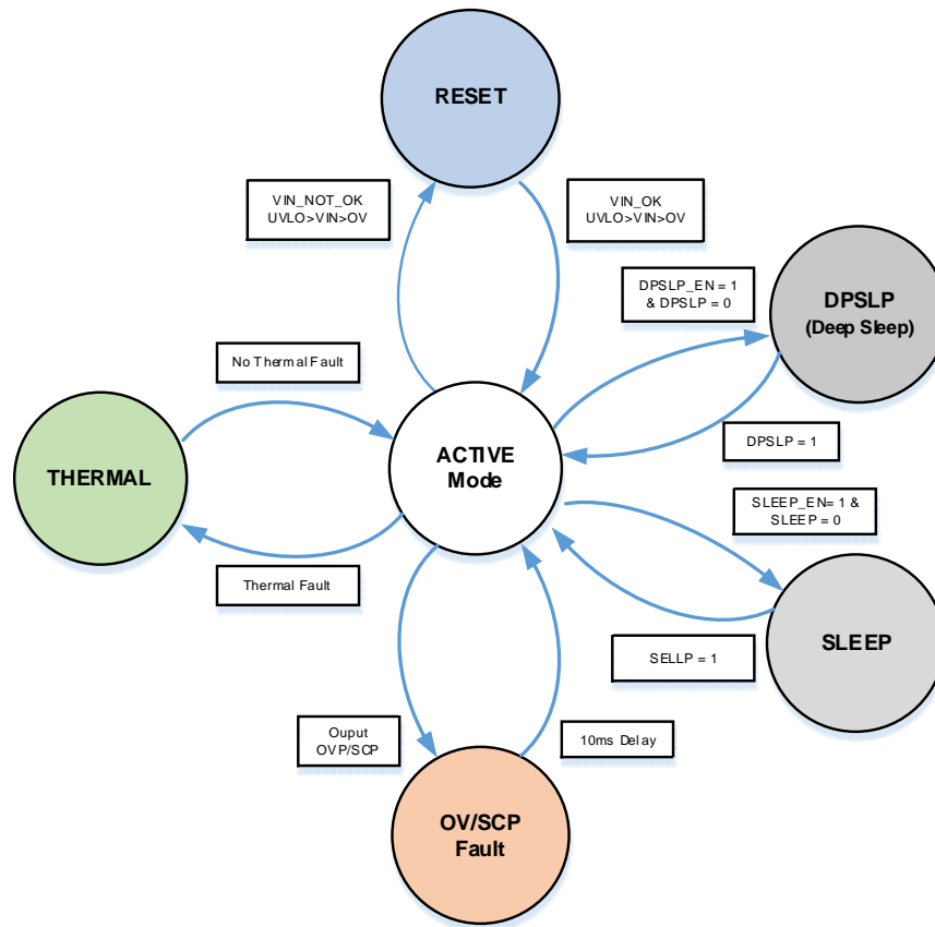
Figure 17. State Machine
