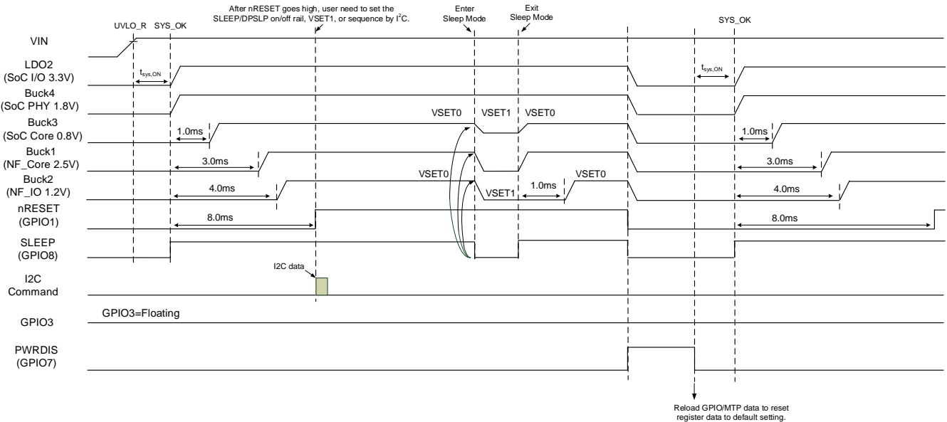
Figure 15. Conceptual of Timing Diagram for PWRDIS during Operating
