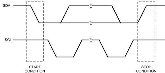
Figure 29. Start and Stop Conditions
