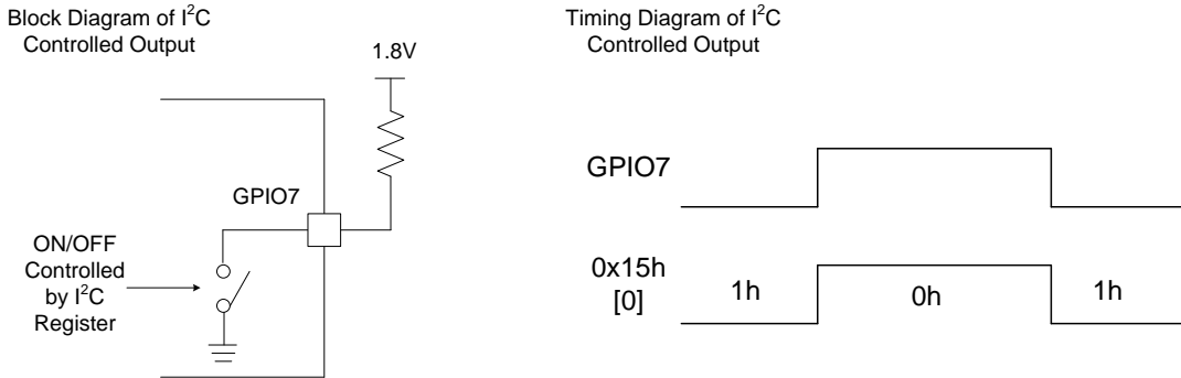
Figure 14. Block Diagram and Timing Diagram of I 2 C Controlled Output Function
