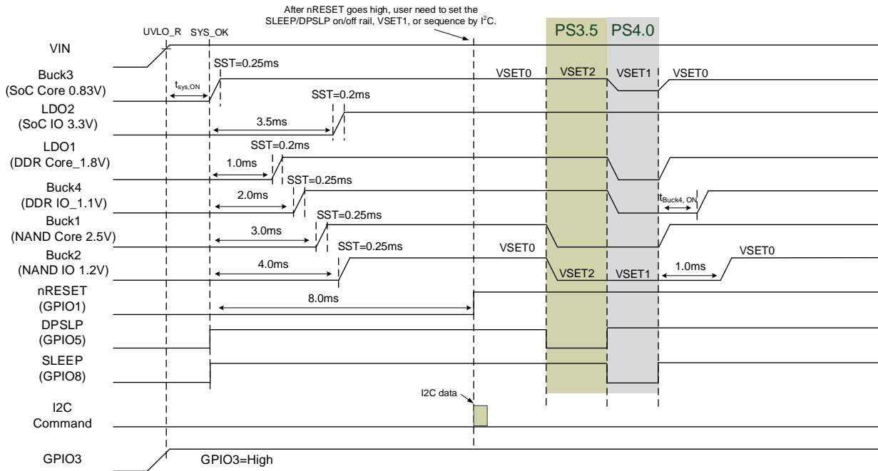
Figure 8. Power Sequence of Sequence A
