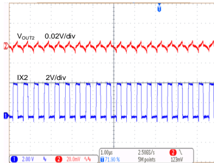
Buck2 Waveforms (FCCM Mode, V_{IN}=3.3V , V_{OUT2}=1.2V , L=0.47\mu H , C_{OUT}=22\mu F , I_{OUT}=2A )
