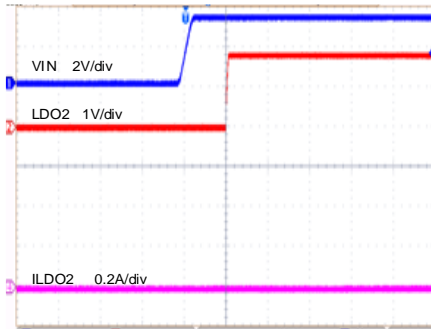
LDO2 Power On ( V_{IN}=3.3V , V_{OUT4}=1.8V , C_{OUT}=1\mu F , I_{OUT}=0A )
