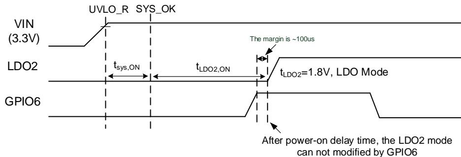
Figure 13. Timing Diagram of GPIO6 Function
