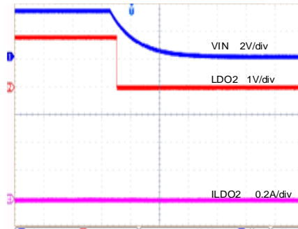
LDO2 Power Off ( V_{IN}=3.3V , V_{OUT4}=1.8V , C_{OUT}=1\mu F , I_{OUT}=0A )
