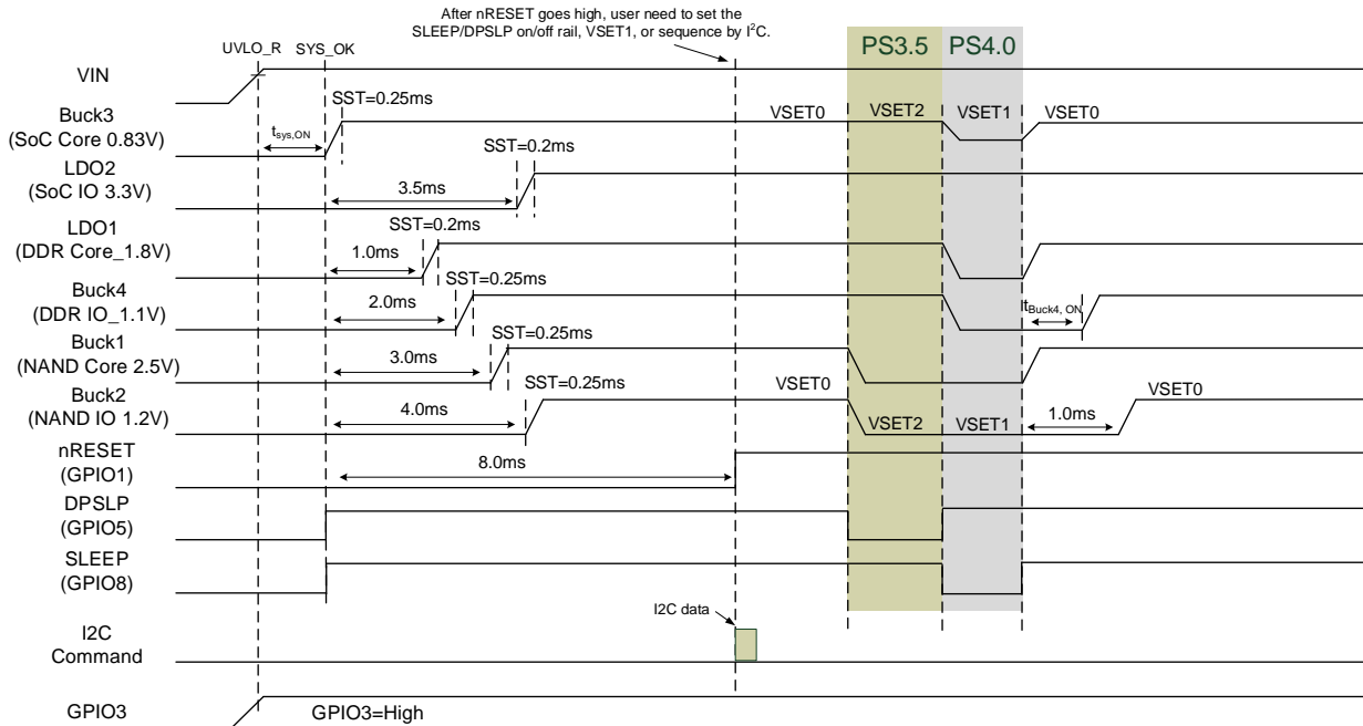
Figure 21. SLEEP and DPSLP Sequence for Application A
