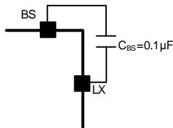
Figure 5. Bootstrap Capacitor Connection
