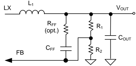
Figure 13. Feed-forward network
