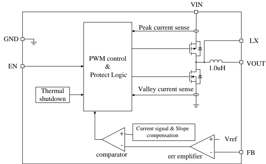
Figure 2. Block Diagram
