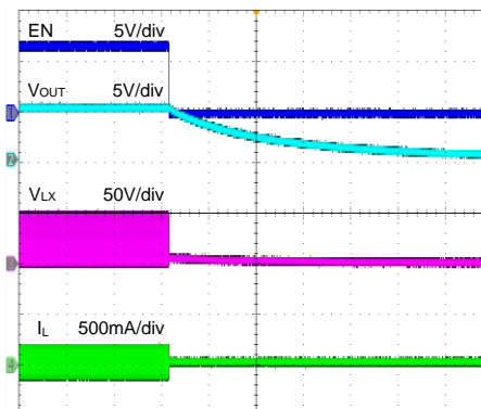
Time (400ms/div)
