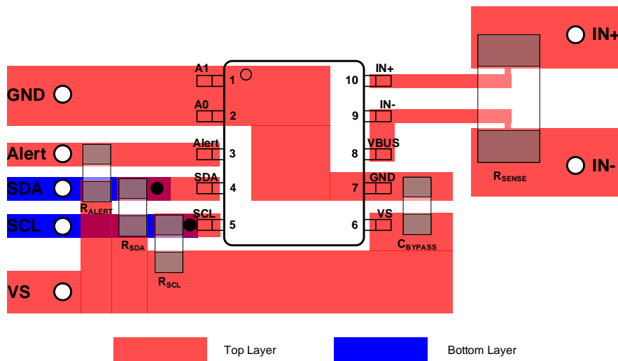
Figure 9. Recommended Layout
