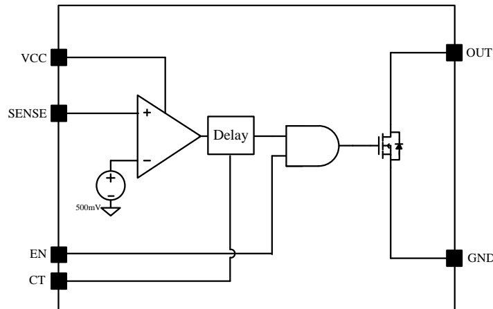
Figure2. Block Diagram
