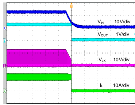
Time (20ms/div)
