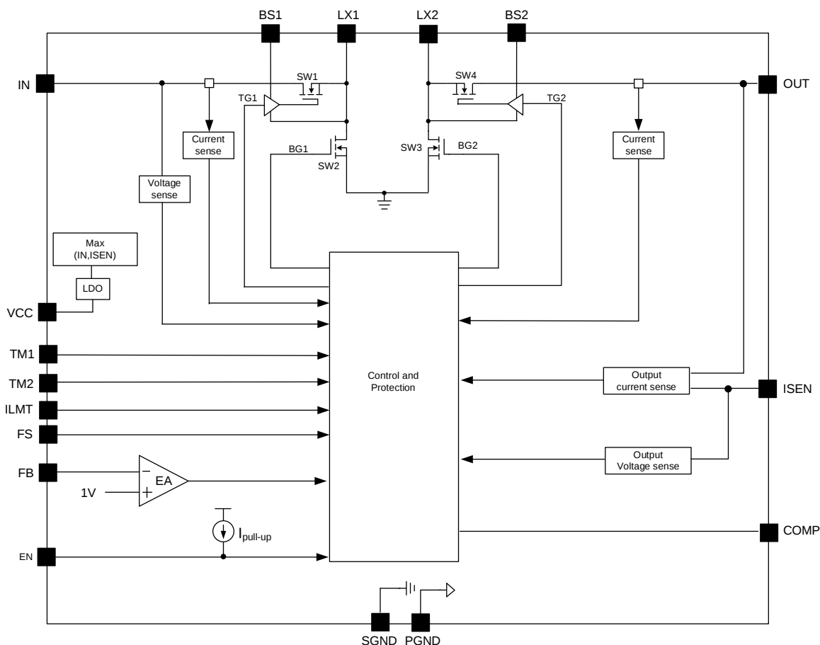
Fig.3 Block Diagram
