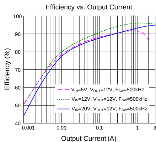
Fig.2 Efficiency vs. Output Current
