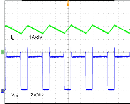
Time (1µs/div)
