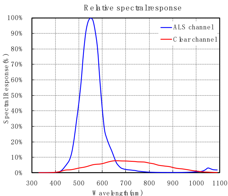
Figure 4. Spectral Responses of SY3079AS22-J01
