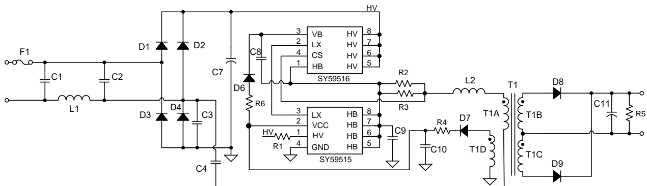
Figure.1c Typical Application
