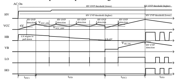
Fig.3 Start up Process of SY59516 and SY59515
