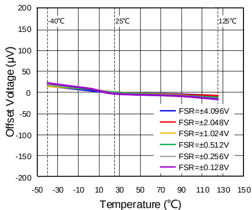
Differential Offset Voltage vs. Temperature
