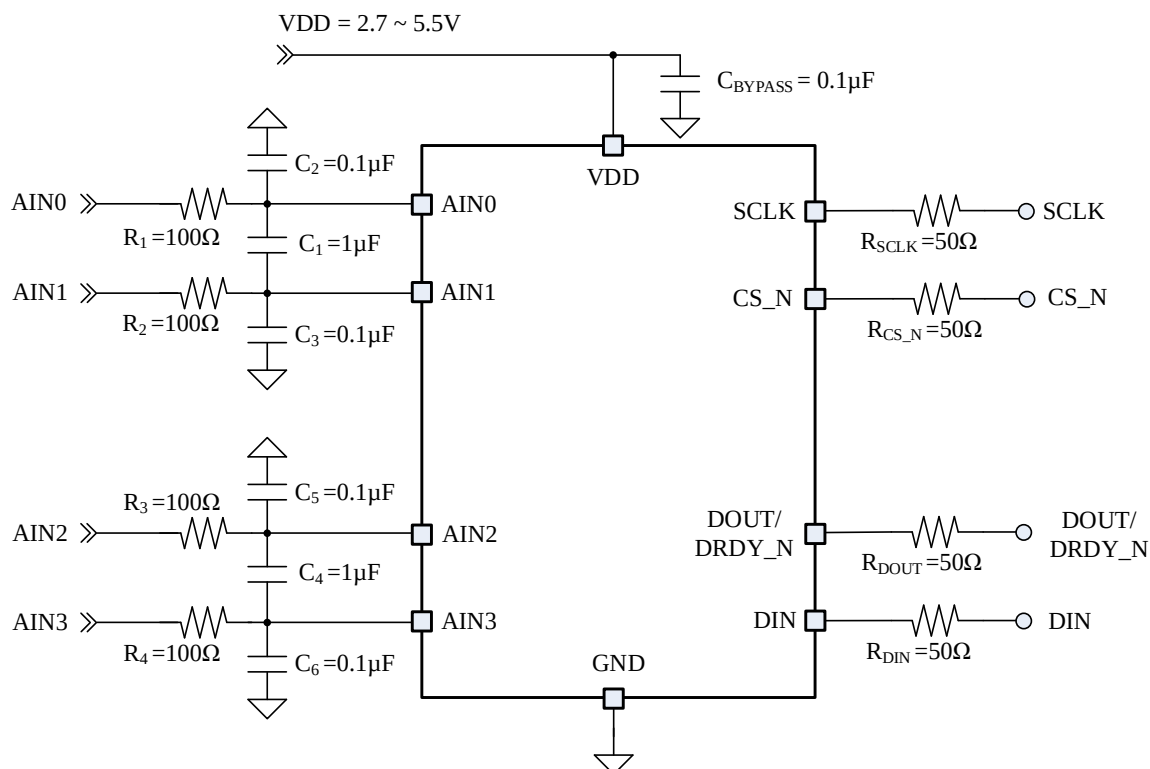
Figure 9. Schematic Diagram
