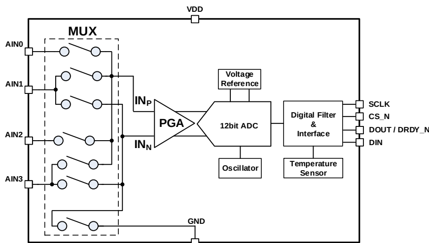
Figure 2. Block Diagram
