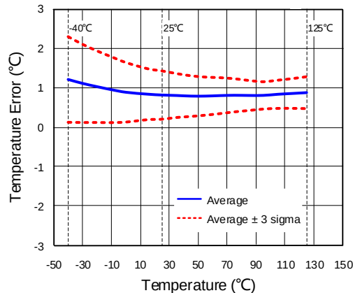
Temperature Sensor Error vs. Temperature
