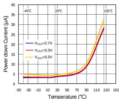
Power down Current vs. Temperature
