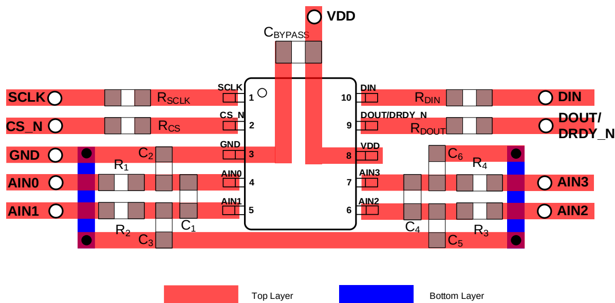
Figure 10. Layout Recommendation
