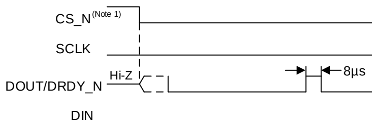
Figure 3. DOUT/DRDY_N Behavior without Data Retrieval in Continuous-Conversion Mode
