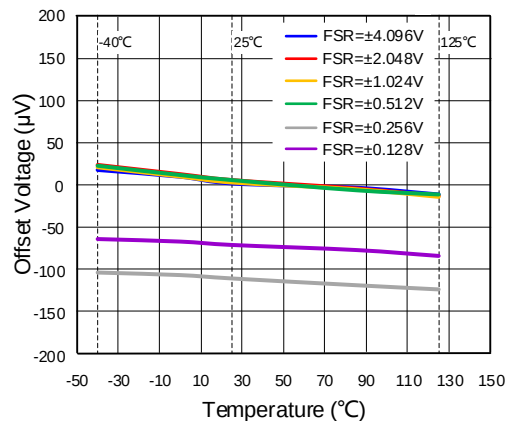
Single-Ended Offset Voltage vs. Temperature
