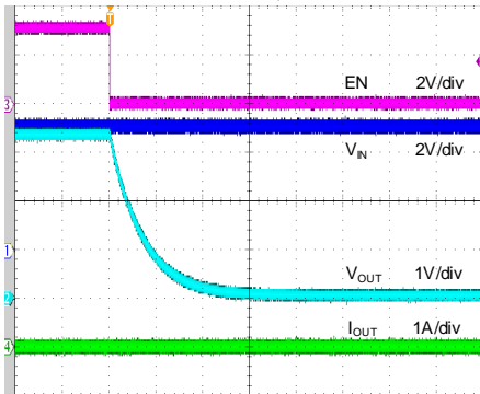
Time (4ms/div)
