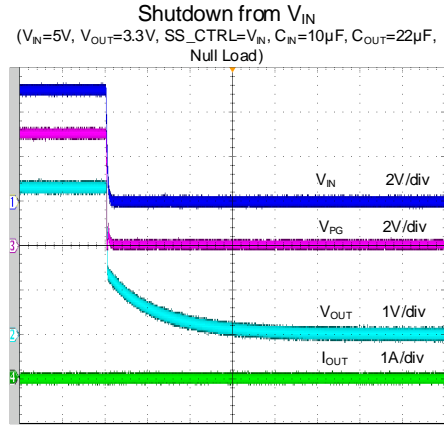
Time (1s/div)
