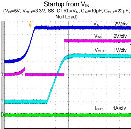
Time (40μs/div)
