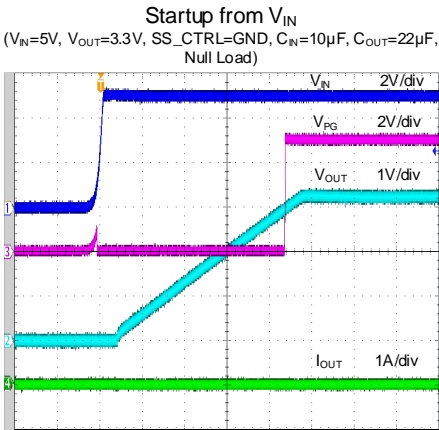
Time (200μs/div)
