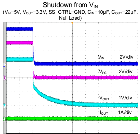
Time (1s/div)
