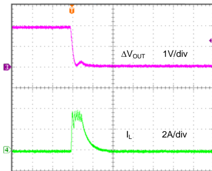
Short Circuit Protection ( V_{IN}=5.0V , V_{OUT}=1.8V , I_{LOAD}=0A -Short)
