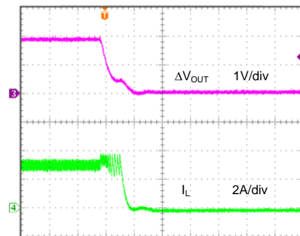
Short Circuit Protection ( V_{IN}=5.0V , V_{OUT}=1.8V , I_{LOAD}=3.0A -Short)
