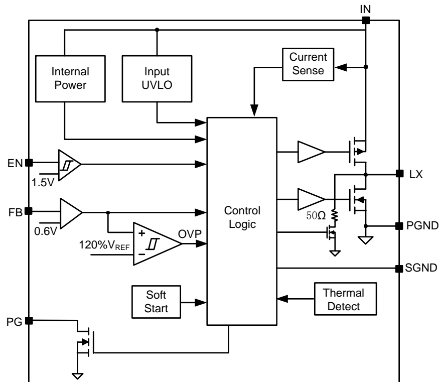
Figure3. Block Diagram
