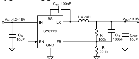
Figure1. Schematic Diagram
