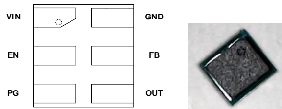
Package:MDFN1.9x1.75-6, Height: 1.08mm max
