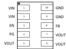
Package:MQFN2.5x2-10, Height: 1.22mm max
