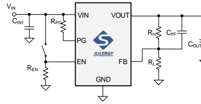
Typical Schematic
