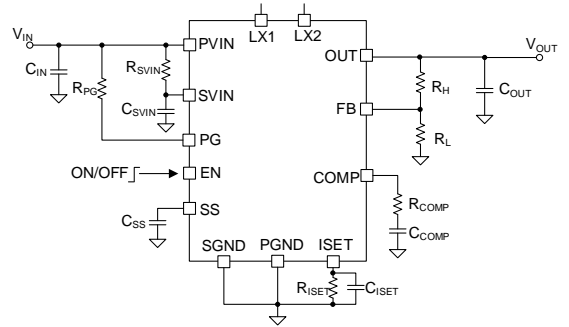
Typical Schematic
