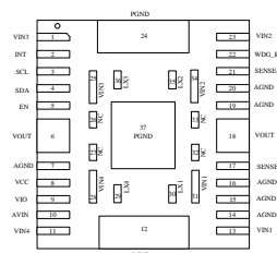
Package:MQFN5x6-24, Height: 1.8mm max
