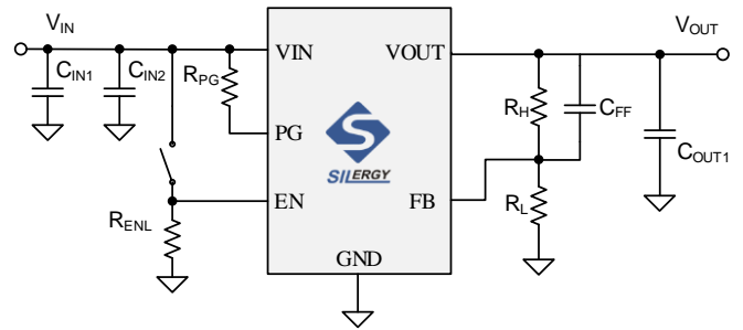
Typical Schematic
