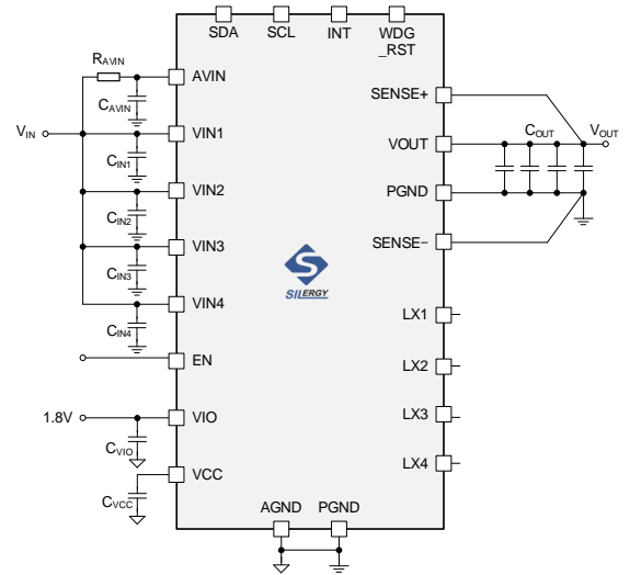
Typical Schematic
